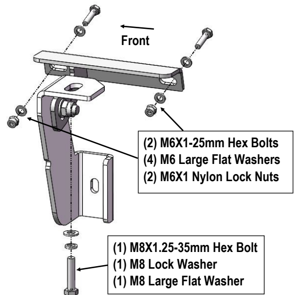
(Fig 6) Assembled Passenger Rear Mounting Bracket Installation
