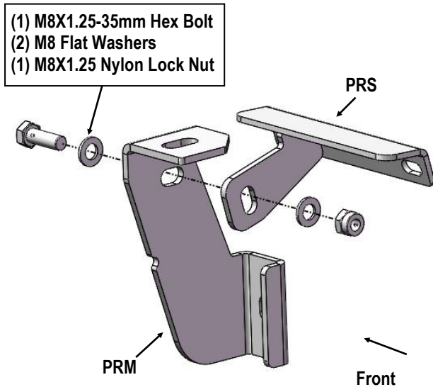
(Fig 4) Passenger Rear Mounting Bracket Assembly
