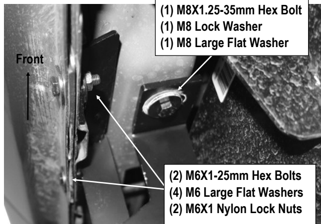
(Fig 3) Passenger Front Mounting Bracket Installed
