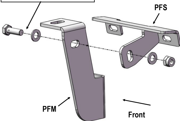
(Fig 1) Passenger Front Mounting Bracket Assembly
