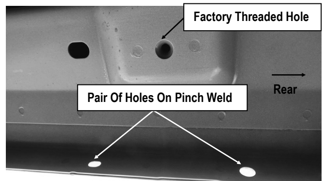
(Fig 5) Passenger Side Rear Mounting Location
