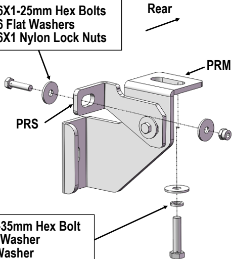
(Fig 7) Passenger Rear Bracket Installed
