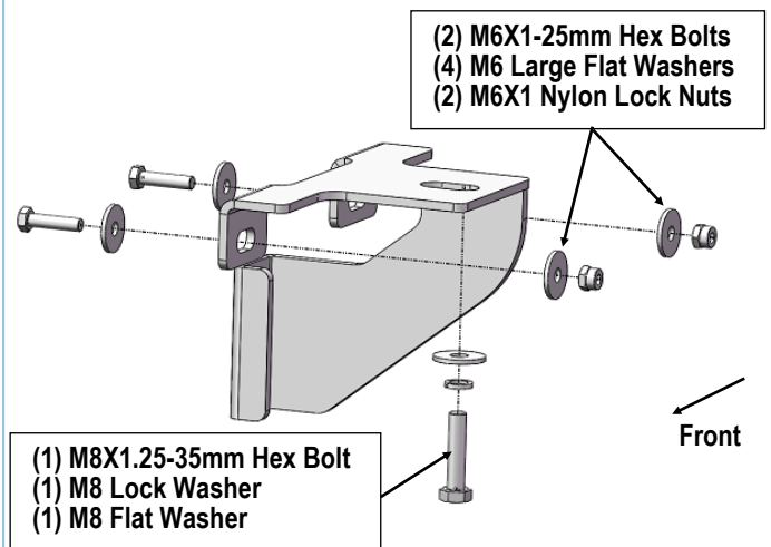
(Fig 2) Passenger Front Mounting Bracket Installed
