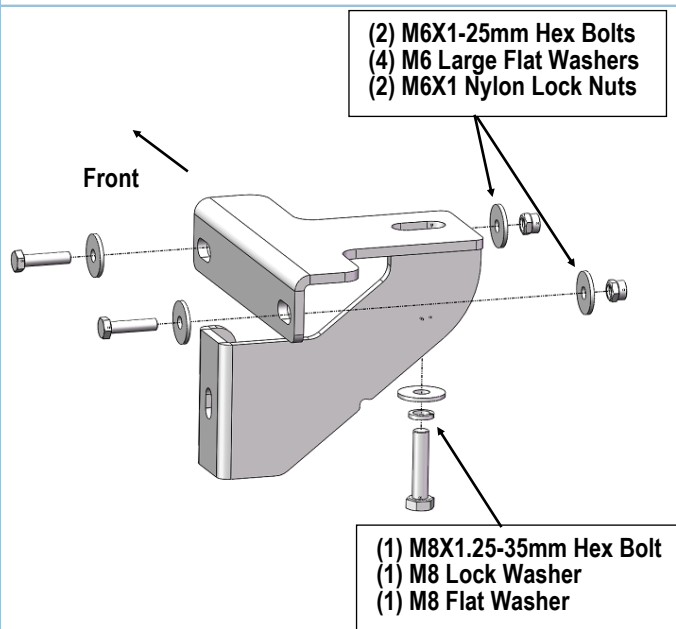
(Fig 4) Passenger Center Mounting Bracket Installed
