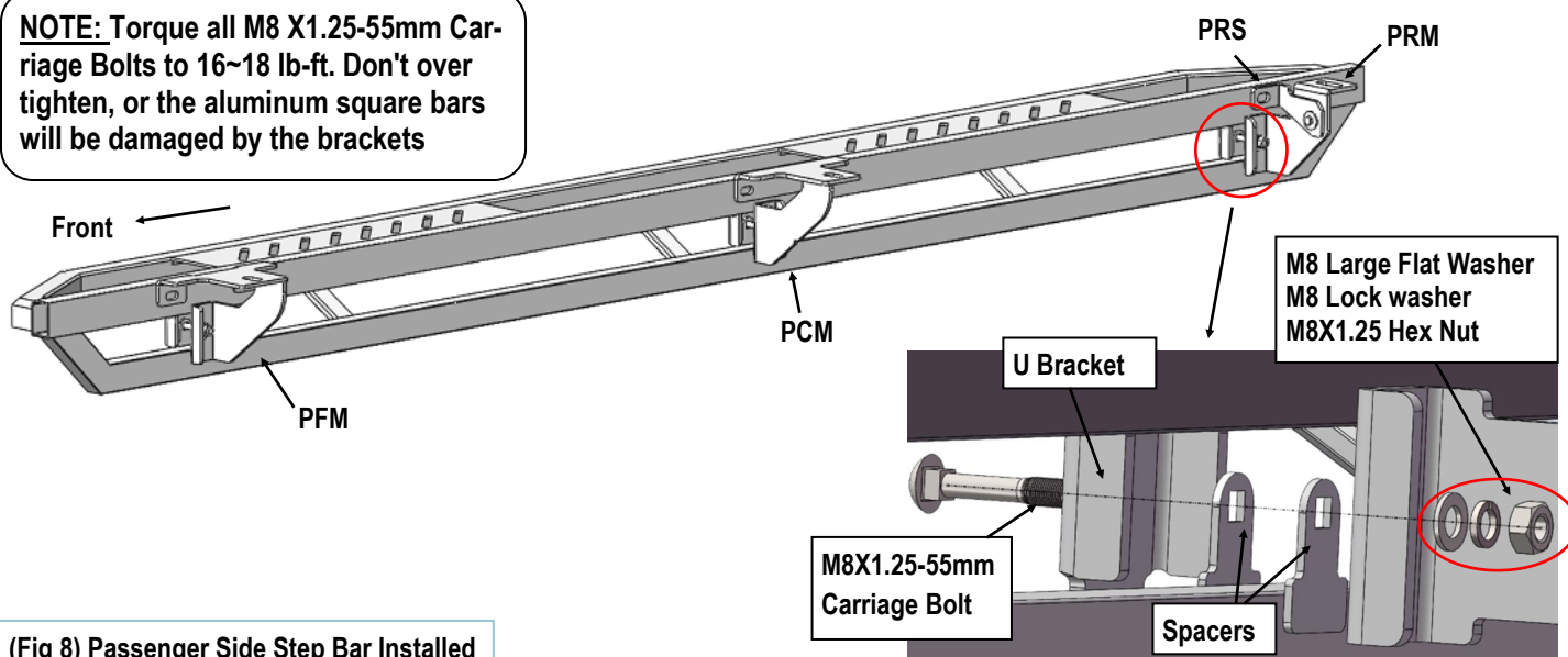
(Fig 8) Passenger Side Step Bar Installed
