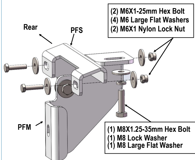
(Fig 4) Passenger Side Front Brackets Installation Pictured
