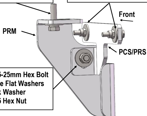
(Fig 8) Passenger Side Rear Brackets Installation Pictured
