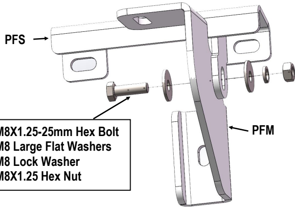
(Fig 3) Passenger Front Mounting Bracket (PFM) and Passenger Front Support Bracket (PFS) Assembly
