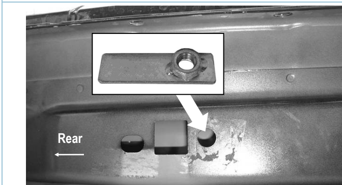
(Fig 3) Passenger Side Rear Mounting Location (Vehicles with open mounting location)
