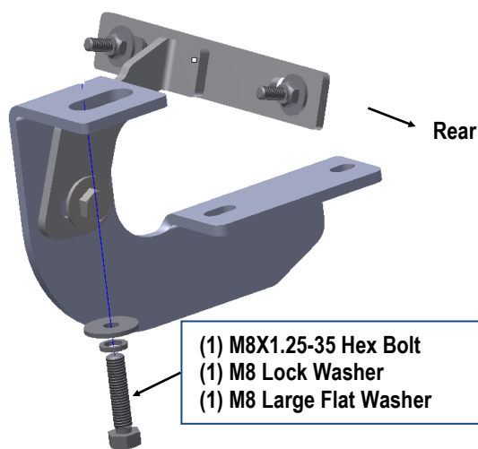
(Fig 10) Passenger Front Mounting Bracket Installed (Vehicles with factory threaded hole in floor panel)
