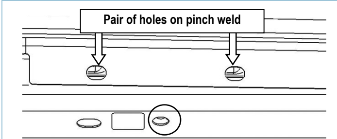
(Fig 2) Line up Nut Plate with hole located between the (2) holes on the pinch weld
