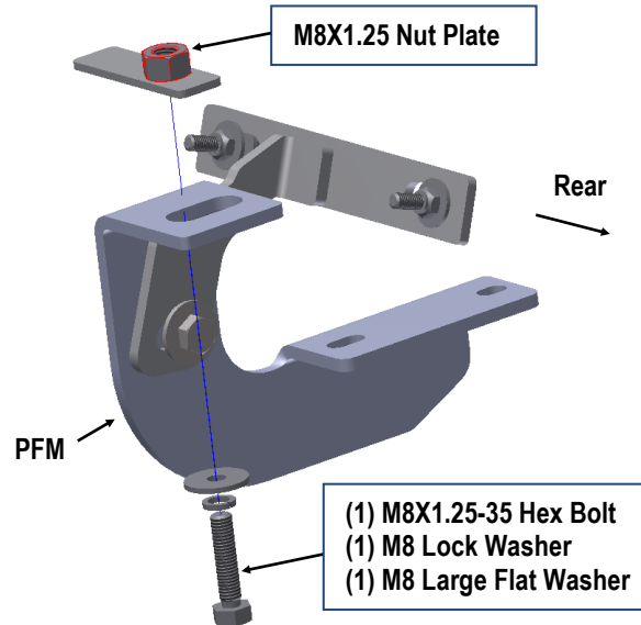
(Fig 9) Passenger Front Mounting Bracket Installed (Vehicles with open mounting location)
