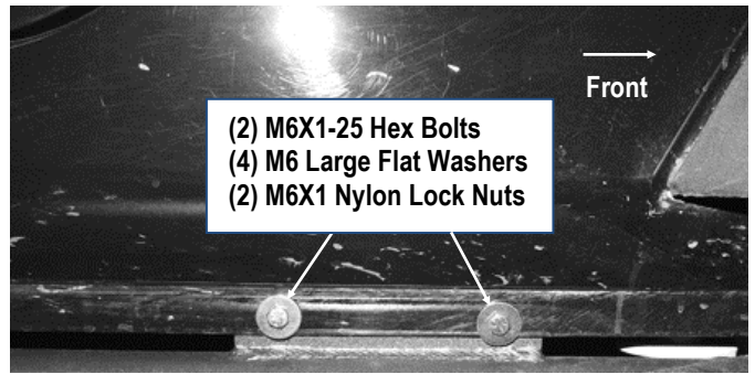
(Fig 8) Passenger Front Support Bracket Installed
