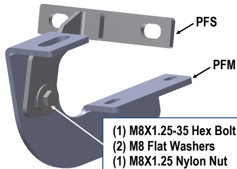
(Fig 6) Passenger Front Mounting Bracket Assembly
