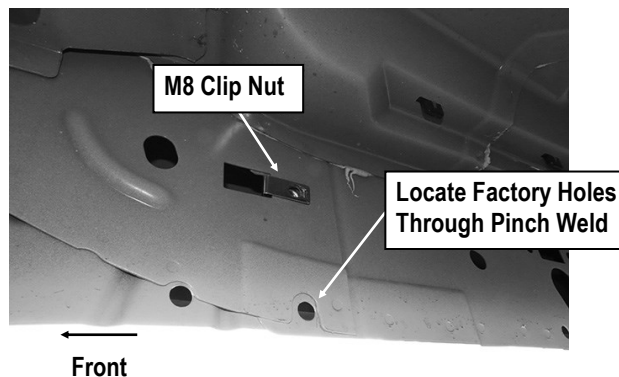
(Fig 3) Slide M8 Clip Nut Into Rectangular Opening
