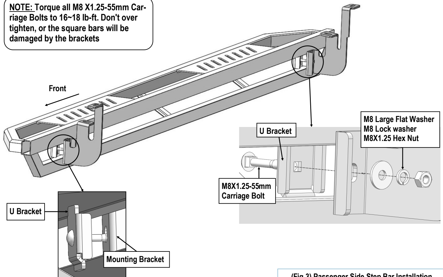
(Fig 3) Passenger Side Step Bar Installation
