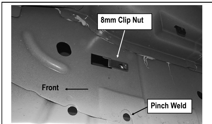
(Fig 3) M8 Clip Nut Installed (On Passenger Front Mounting Location)
