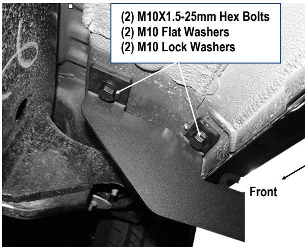
(Fig 3) Passenger Front Mounting Bracket Installed
