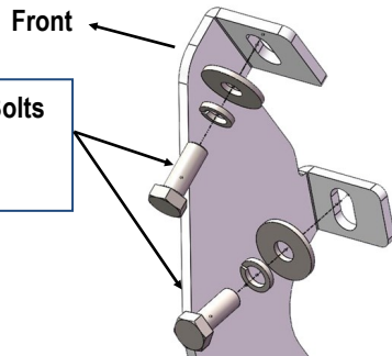
(Fig 2) Passenger Front Mounting Bracket Installed
