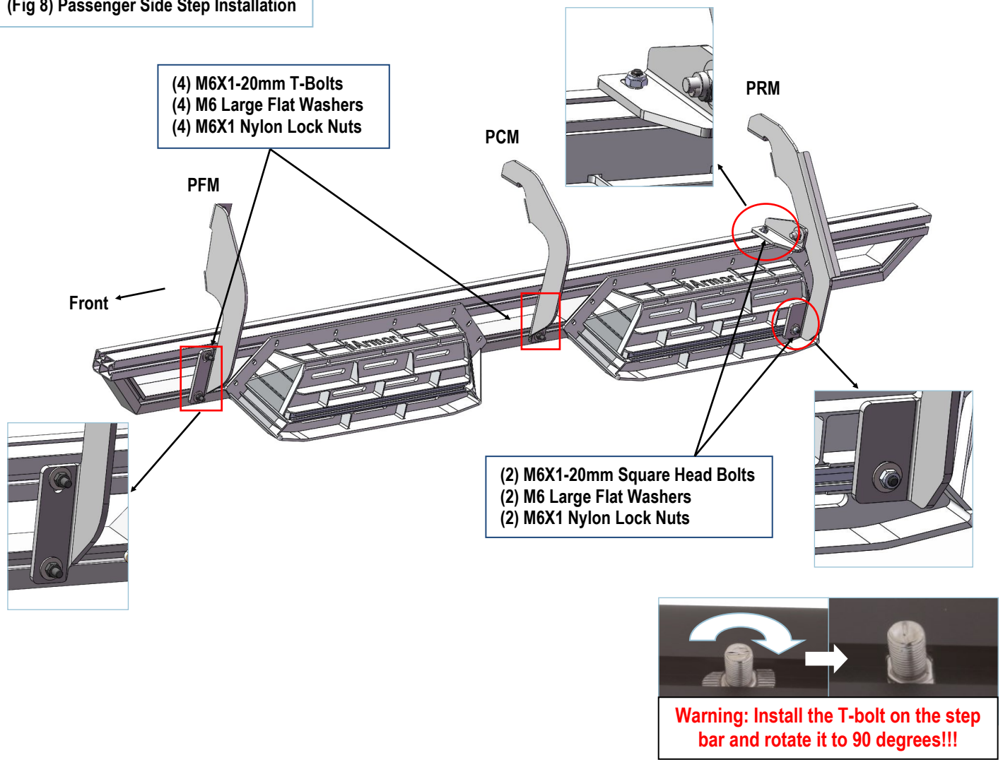
(Fig 8) Passenger Side Step Installation
