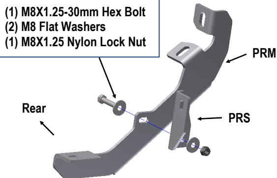
(Fig 7) Passenger Rear Support Bracket Installed
