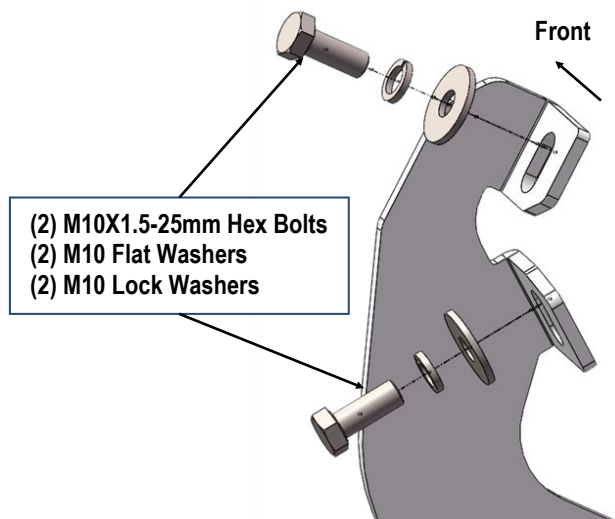
(Fig 5) Passenger Center Mounting Bracket Installed
