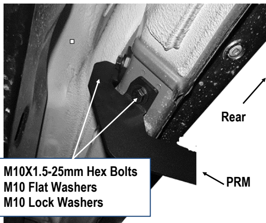
(Fig 6) Passenger Rear Mounting Bracket Installed
