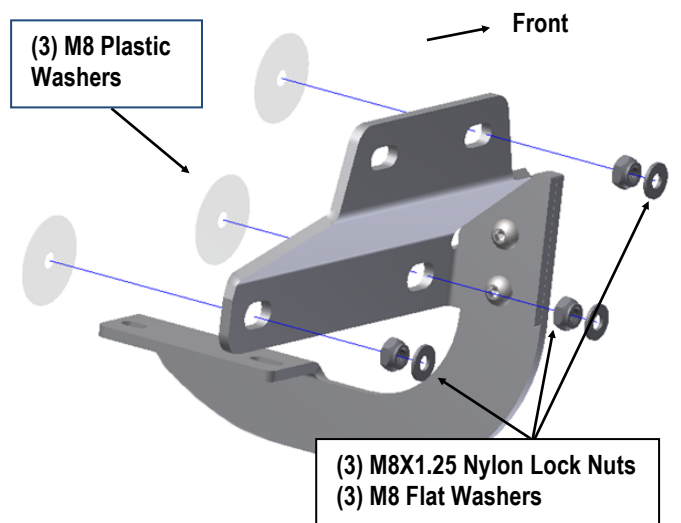
(Fig 3) Driver Side Front Mounting Bracket Installed
