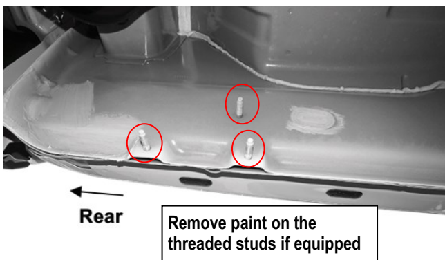
(Fig 5) Driver Rear Mounting Location
