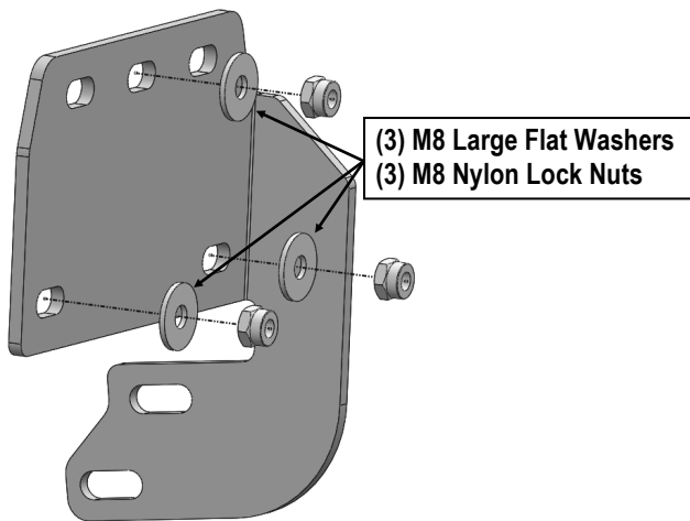
(Fig 4) Driver Center Mounting Bracket Installation
