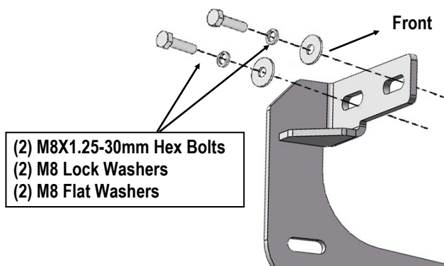
(Fig 9) Driver Front Mounting Bracket Installed (Models w/ factory installed threaded inserts/M8 Bolt/Nut Plate not required)
