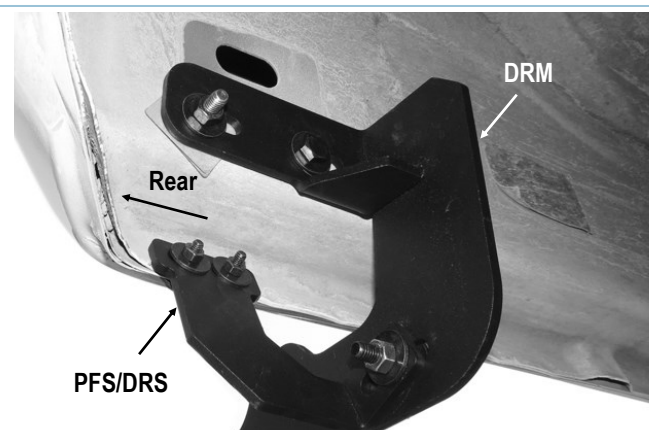
(Fig 14) Driver Rear Brackets installed
