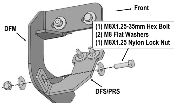
(Fig 10) Attach Driver Front Support Bracket to Drive Front Mounting Bracket
