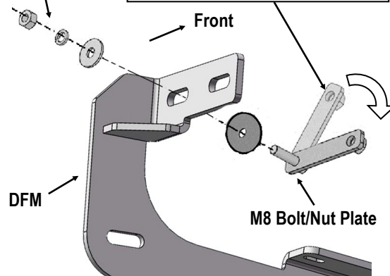
(Fig 7A) Attach Driver Front Mounting Bracket to M8 Bolt/Nut Plate
