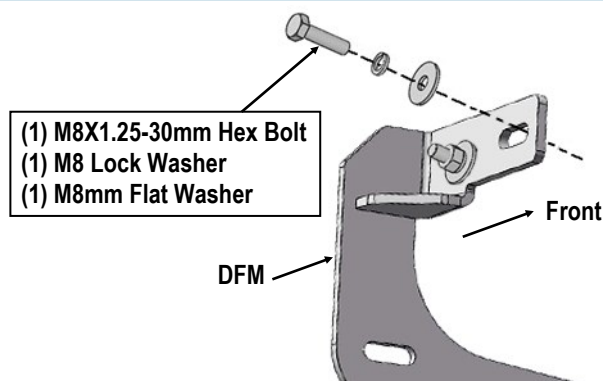
(Fig 7B) Attach Driver Mounting Bracket to threaded end of the M8 Bolt/Nut Plate
