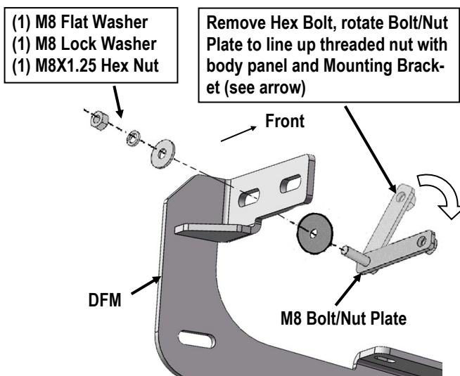
(Fig 7A) Attach Driver Front Mounting Bracket to M8 Bolt/Nut Plate
