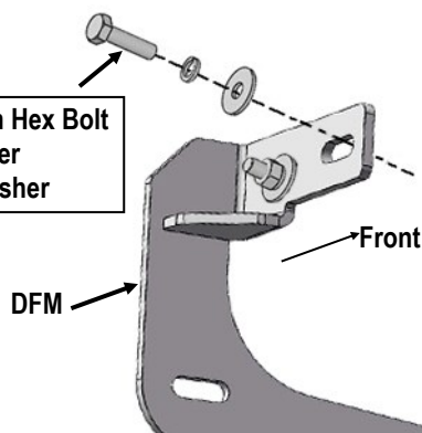
(Fig 7B) Attach Driver Mounting Bracket to threaded end of the M8 Bolt/Nut Plate
