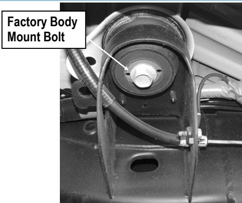
(Fig 1) Remove Factory Body Mount Bolt
