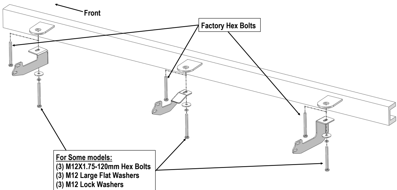
(Fig 2) Driver Side Mounting Brackets Installation
