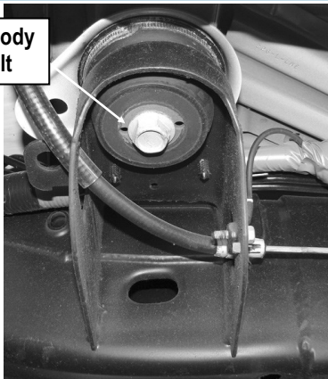
(Fig 1) Remove Factory Body Mount Bolt
