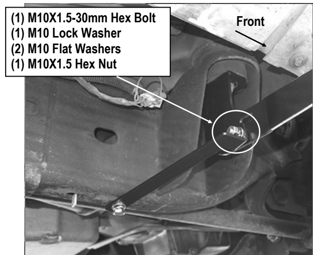
(Fig 7) Passenger Front Support Bracket Installation (For Up to 2007 2500/3500 Models)
