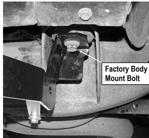
(Fig 2) Passenger Front Mounting Bracket (PFM) Installed
