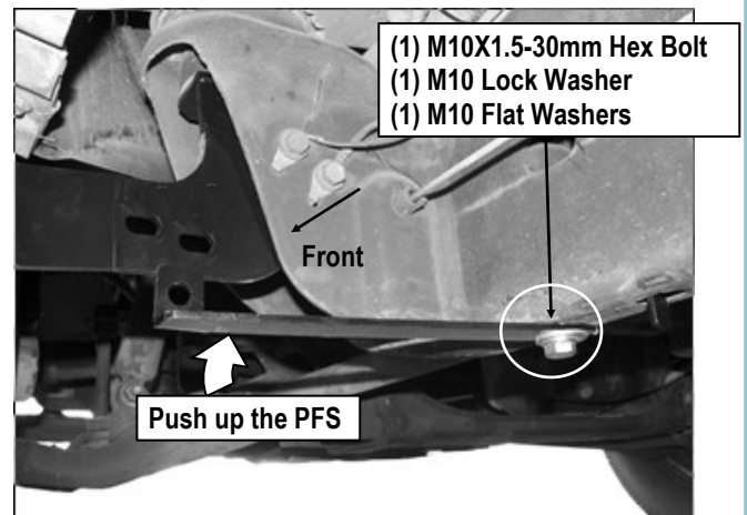
(Fig 6) Passenger Front Support Bracket Installation (For Up to 2007 2500/3500 Models)
