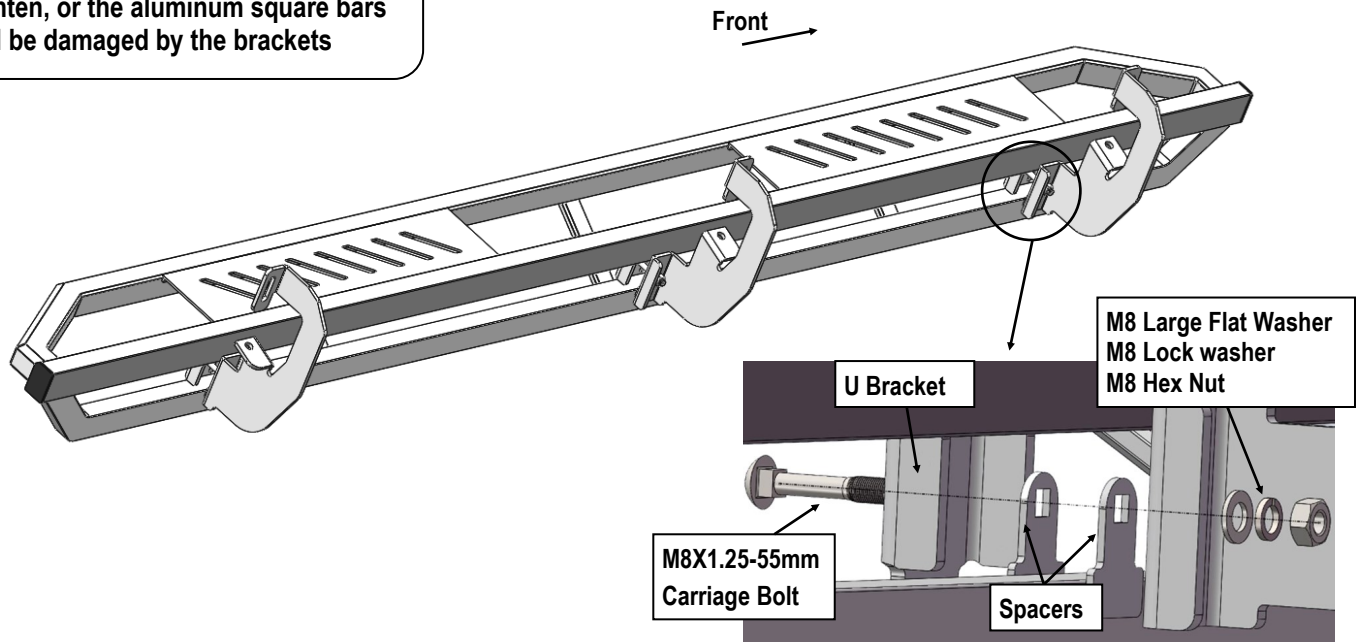
(Fig 3) Driver Side Step Bar Installed
