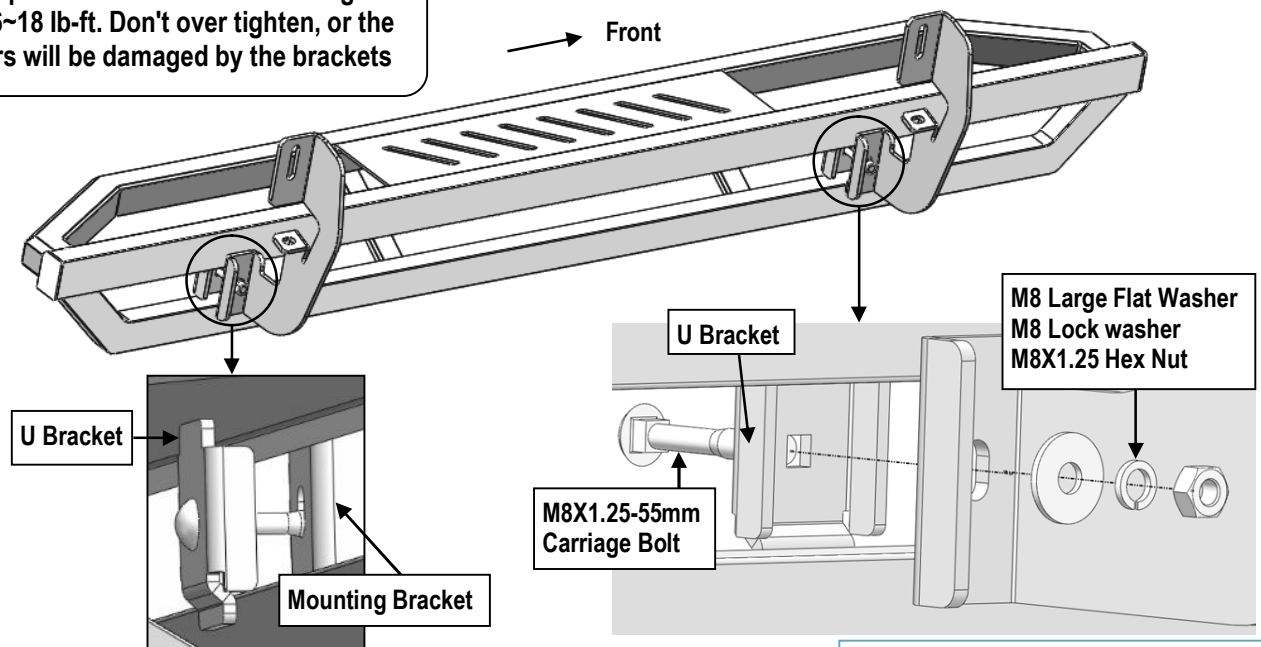
(Fig 6) Driver Side Step Bar Installation
