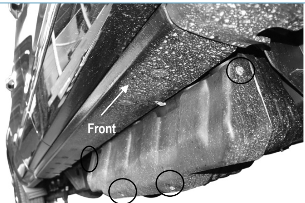
(Fig 9A) 17-on Passenger side pictured with DEF plastic tank cover. Remove (4) hex bolts to remove plastic cover
