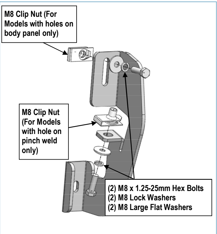
(Fig 5) Driver Front Mounting Bracket Installation
