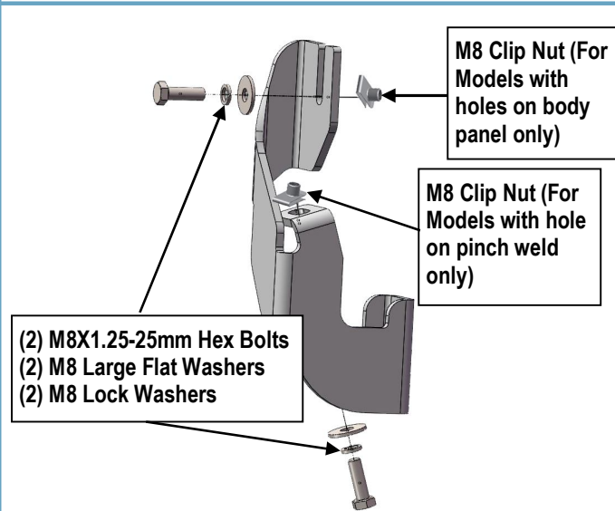
(Fig 10) Passenger Front Mounting Bracket Installation
