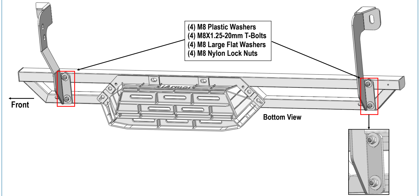
(Fig 10) Passenger Side Step Installation
