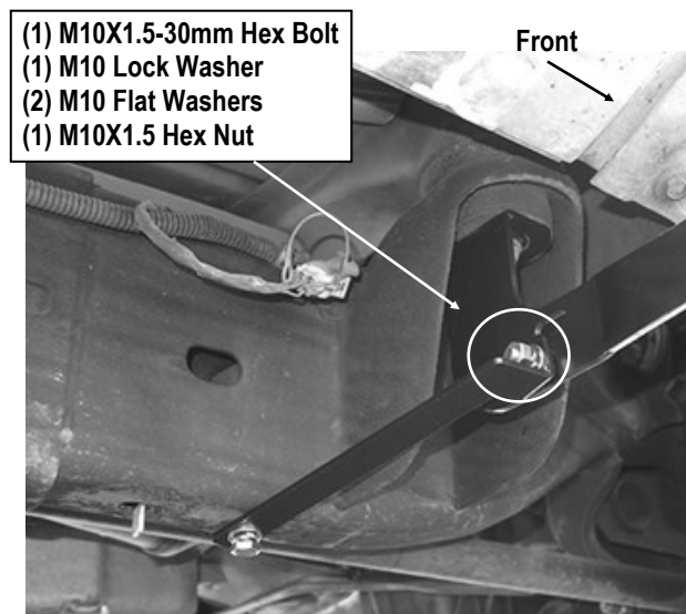
(Fig 6) Passenger Front Support Bracket Installation (For Up to 2007 2500/3500 Models)
