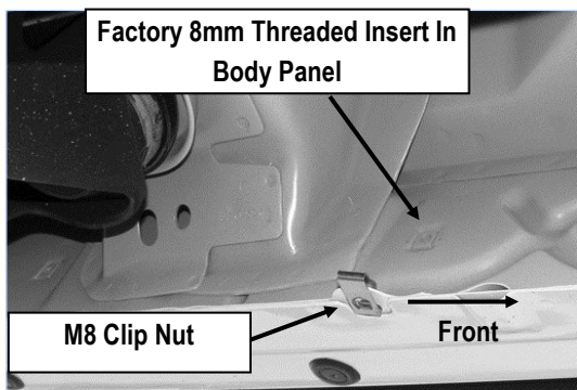
(Fig 5) Driver Side Center Mounting Location
