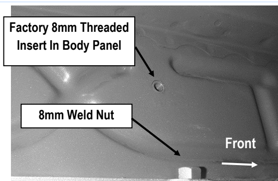
(Fig 4) Driver Side Front Mounting Location
