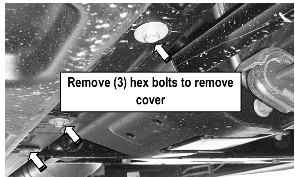
(Fig 11) 07-16 Passenger Side Front Pictured with DEF Tank Cover.
