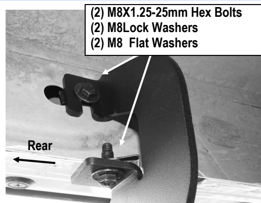
(Fig 9) Driver Center Bracket Installed
