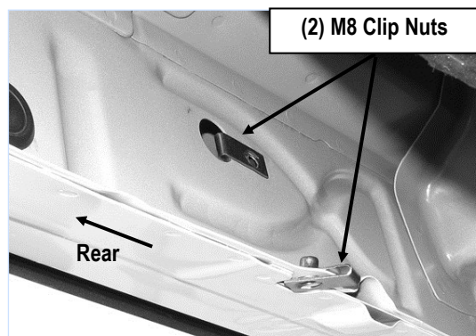
(Fig 7) Driver Side Rear Mounting Location
