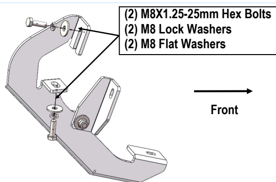
(Fig 8) Driver Front Bracket Installed
