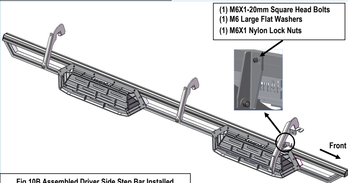
Fig 10B Assembled Driver Side Step Bar Installed
