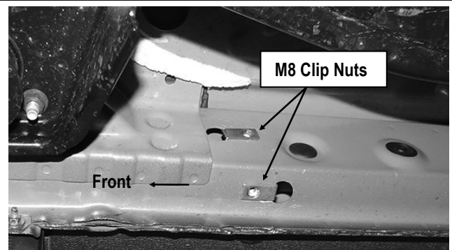
(Fig 3) M8 Clip Nuts Installed (on the Passenger Side Front Mounting Location)
