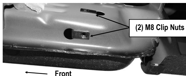
(Fig 7) Passenger Side Rear Mounting Location
