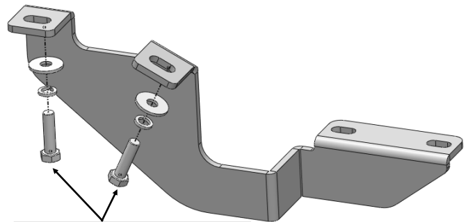
(Fig 1) Passenger Side Front Mounting Location
