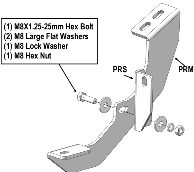
(Fig 5) Passenger Side Rear Brackets Assembly
