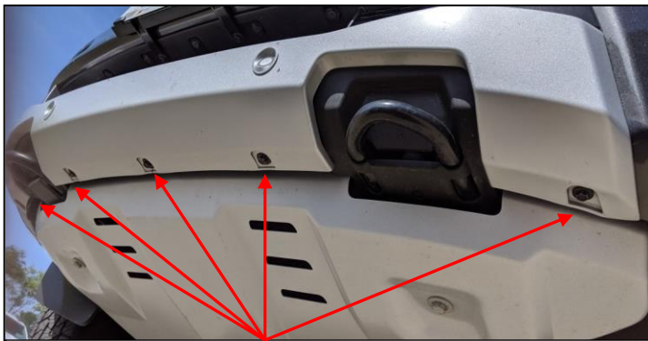
(Fig 1) Five Lower Valance Bolts
